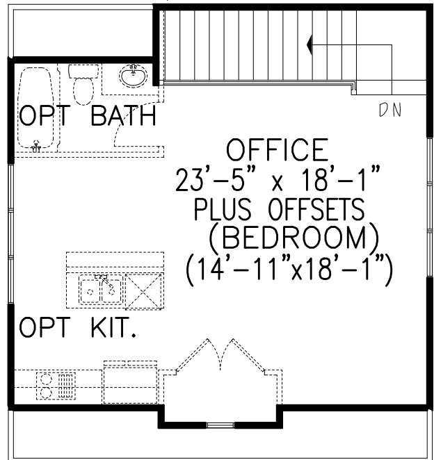
2nd FLOOR PLAN OFFICE 460 SQ. FT.
