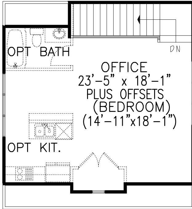
2nd FLOOR PLAN OFFICE 460 SQ. FT.
