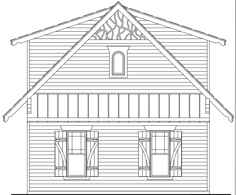
© 2019 GARRELL ASSOCIATES, INC. 19099 FRONT ELEVATION
