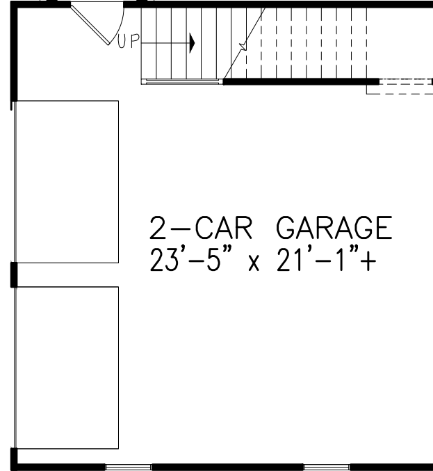
1st FLOOR PLAN GARAGE 624 SQ. FT.
