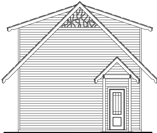
© 2019 GARRELL ASSOCIATES, INC. 19099 REAR ELEVATION
