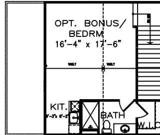
OPTIONAL SECOND FLOOR PLAN 432 SQ. FT.
